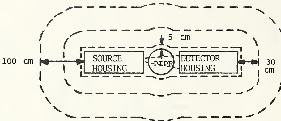
FIGURE IIA. Density Gauge
